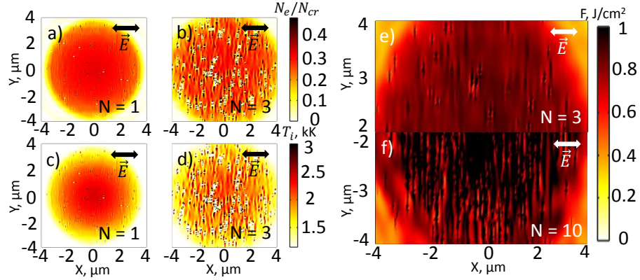
Figure 1: (a-d) Electron density and temperature snapshots of the irradiated regions subject to one pulse N = 1 and few pulses N = 3 irradiation. The maximum values are plotted. The electron density is normalized to the critical value N_{cr} . (e-f) Energy deposition snapshots (in terms of fluence) showing the effect of the number of applied pulses on the ordering of periodic nanoplasmas in the chosen half-Gaussian spots. The pulse energy is 250 nJ, the pulse duration is 200 fs. The number of pulses N is indicated in each image.
