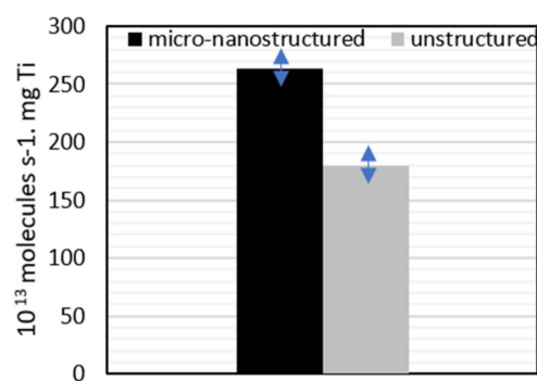
Figure 7. Disappearance rate of FA per \mu\text{g} of Ti obtained for micro-nanostructured and unstructured \text{TiO}_2 films.
