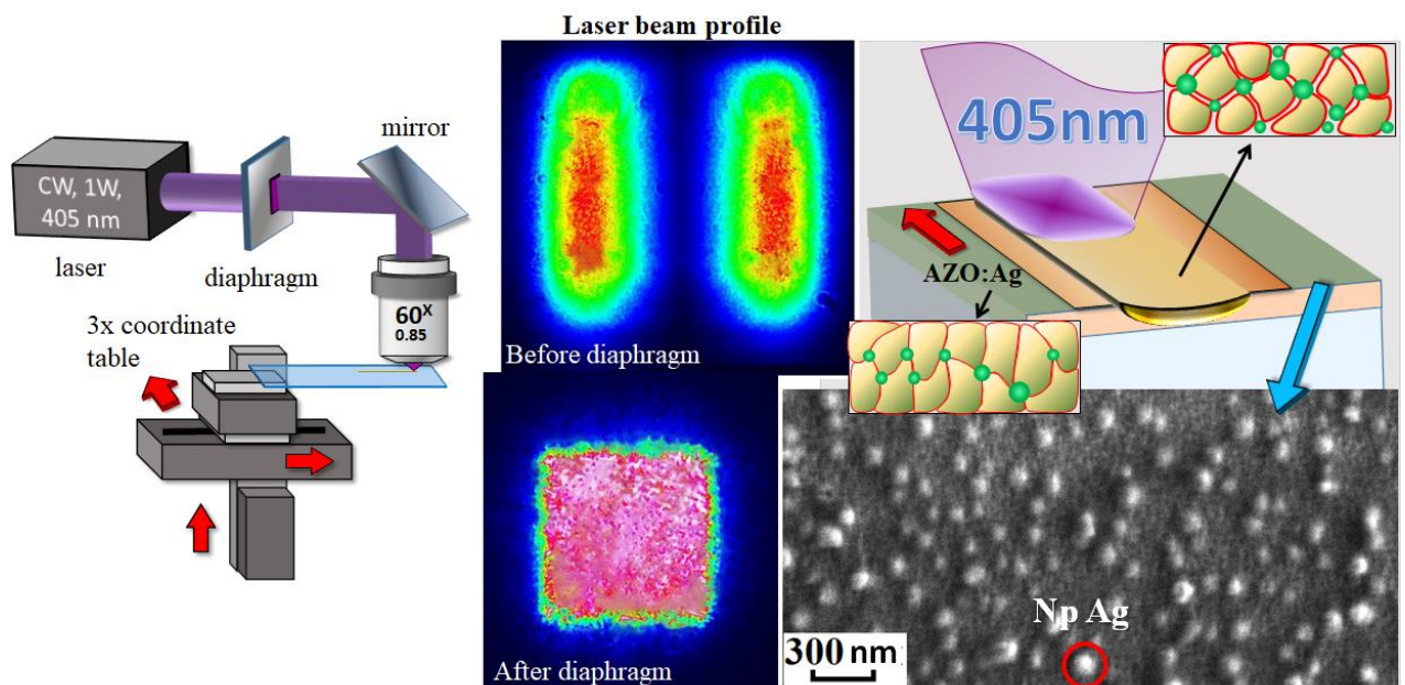
Figure 1. (a) Experimental setup scheme for laser modification of AZO: Ag thin films in the matrix crystallization regime with growth / decomposition of Ag NPs; (b) original film SEM image
