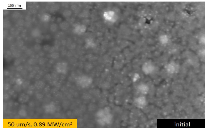
Figure 9. SEM image of the area at the border of the track and the original film
