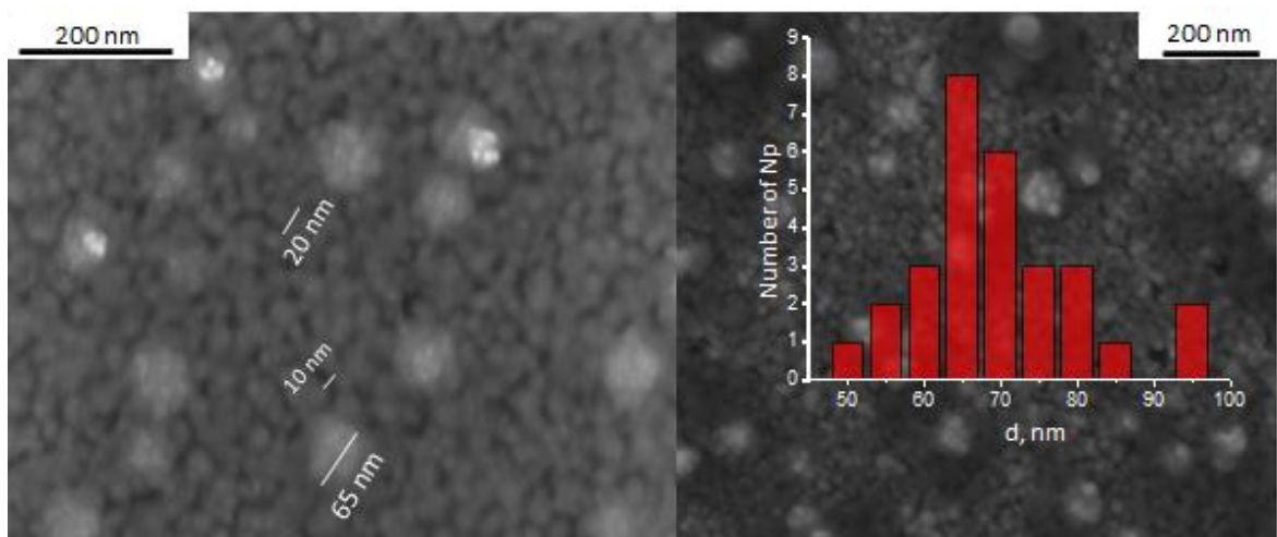
Figure 7. SEM images of the original film and a histogram of Ag NPs size distribution by diametral size
