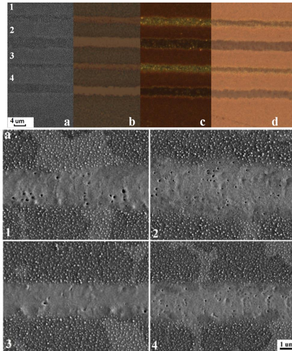
Figure 6. (a) SEM images 1 – 50 \mu\text{m/s} , 0.89 \text{MW/cm}^2 ; 2 – 50 \mu\text{m/s} , 1.07 \text{MW/cm}^2 ; 3 – 100 \mu\text{m/s} , 0.89 \text{MW/cm}^2 ; 4 – 100 \mu\text{m/s} , 1.07 \text{MW/cm}^2 ; optical images in (b) transmitted light of bright field, (c) reflected light of dark field, (d) reflected light of bright field of the recorded track
