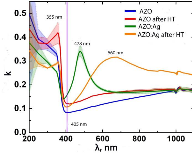
Figure 3. Extinction of AZO and AZO: Ag films without HT and after HT in the furnace
