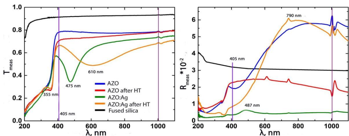
Figure 2. Transmission and reflection of AZO films without HT (blue curve) and after HT in the furnace (red curve), as well as AZO:Ag without HT (green curve) and after HT in the furnace (orange curve)
