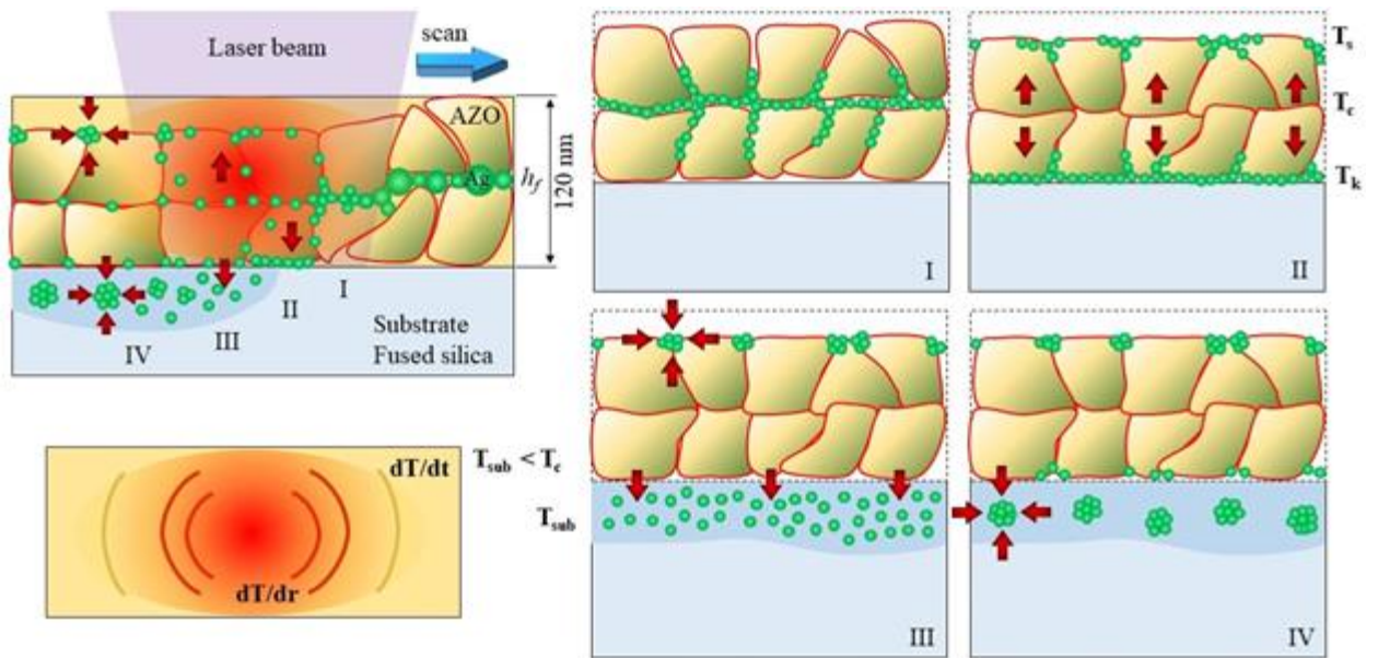
Figure. 11. The scheme of AZO:Ag film photothermal modification with the following stages: I. Decomposition of Ag NPs into monomers; II. mass transfer of Ag monomers from the center of the film to the surface and to the film-substrate interface; III. the outflow of Ag monomers from the film to the substrate during its softening, as well as the growth of Ag nanoclusters on the film surface; IV. agglomeration of Ag monomers and growth of NPs in the substrate.
