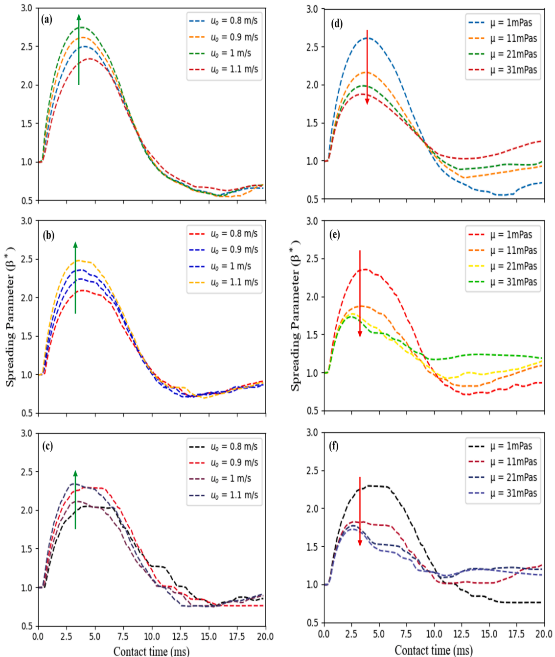
Fig. 8. Spreading parameter ( \beta^* ) at u_o = 0.8\text{m/s} - 1.1\text{m/s} (a) - (c) and \mu = 1\text{mPas} - 31\text{mPas} (d)–(f) for flat, triangular and a two-period relief Ti-6Al-4V alloy surface.
