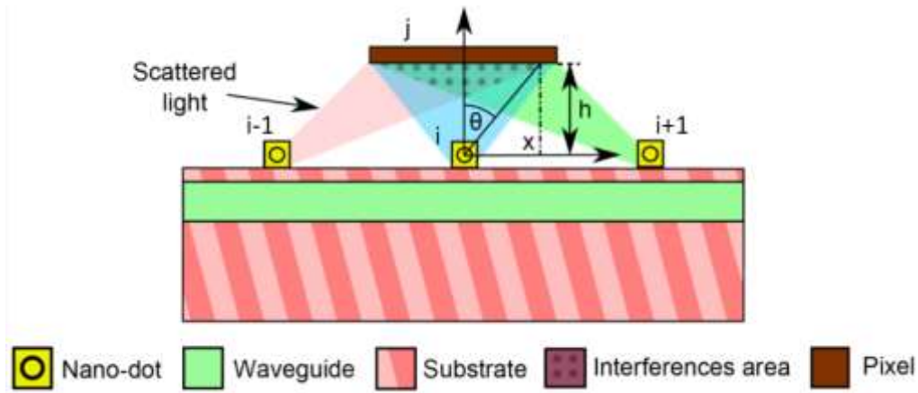
Fig. 4 Schematic view of the scattered light extracted from the sample, and its angular divergence towards the detector, showing the problem of overlapping between too close sampling centers (reproduced from Thomas 2015)
