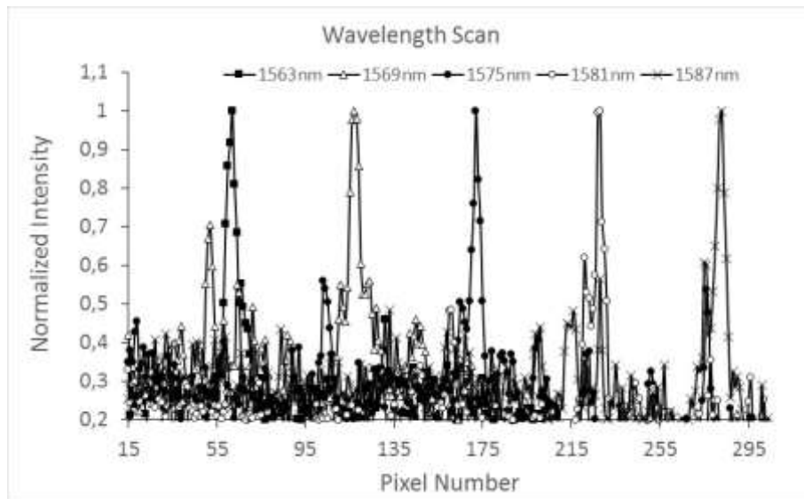
Fig. 27 Detected peak on an array of pixels, as the wavelength is scanned within the source tuning range. Side lobes are visible, due to inhomogeneous grating period fabrication, and induce crosstalk (see for example the secondary lobe at 1569nm (open triangles) close to the main peak at 1563nm (filled squares)), (reproduced from d'Amico 2017)
