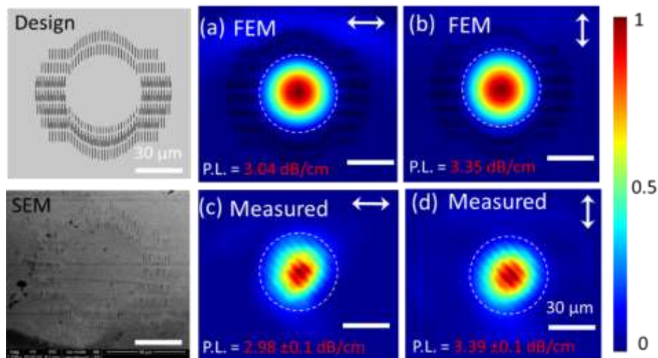
Fig. 2 Simulation and experiment of the Type II laser written waveguide: Comparison of near field TE and TM modes. Interference fringes in the measured mode images are due to back-reflections in the optical guiding imaging system (reproduced from Huu-Dat 2017)
