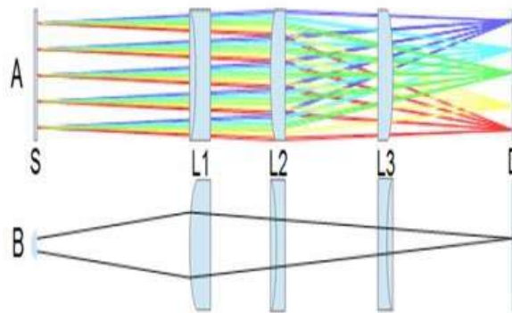
Fig. 26 Experimental Set-Up using a lens triplet, allowing for angular discrimination of the different wavelengths in the optical beam. (A) Sketch of optical rays along the vertical waveguide propagation axis. (B) Front view sketch, showing how the angular divergence of the signal extracted is focused on the detector (from d’Amico2017).
