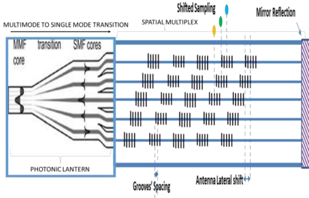
Fig. 15 Basic principle of a spatial multiplexer based on a collecting photonic lantern, followed by a set of parallel waveguides with the shifted sampling centers
