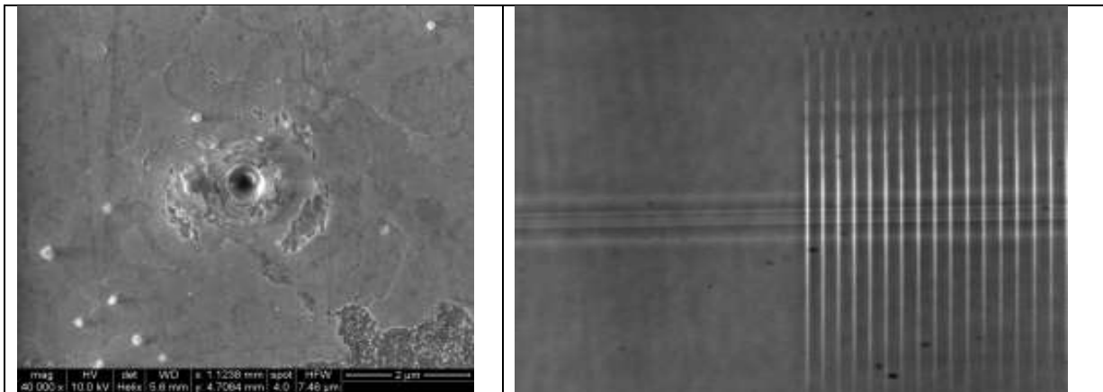
Fig. 3 Front view (left) of a Bessel void, using MEB imaging. Top view (right), using simple microscopy, of a set of Bessel voids transverse to the waveguide (reproduced from Martin16)
