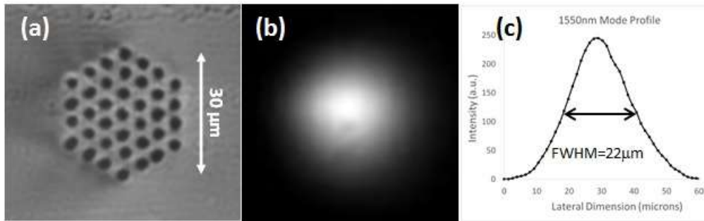
Fig. 1 (a) Multicore hexagonal single mode waveguide fabricated in GLS using short laser pulses. (b) Image of the mode obtained using a 1550nm SLED (same scale as (a)) and (c) mode profile showing large FWHM (reproduced from d’Amico 2017)
