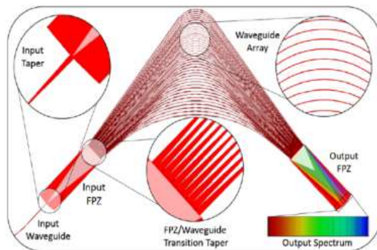
Fig. 20 Principle of an Arrayed Waveguide Grating (reproduced from Douglass 2015)
