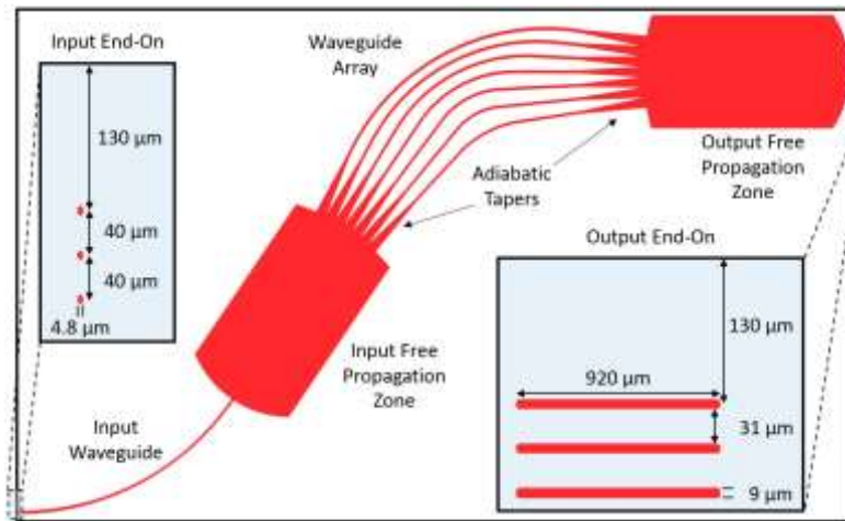
Fig. 21 Top down schematic of a three layered AWG sample. Inserts show the input and output end-on (reproduced from Douglass 2018B).
