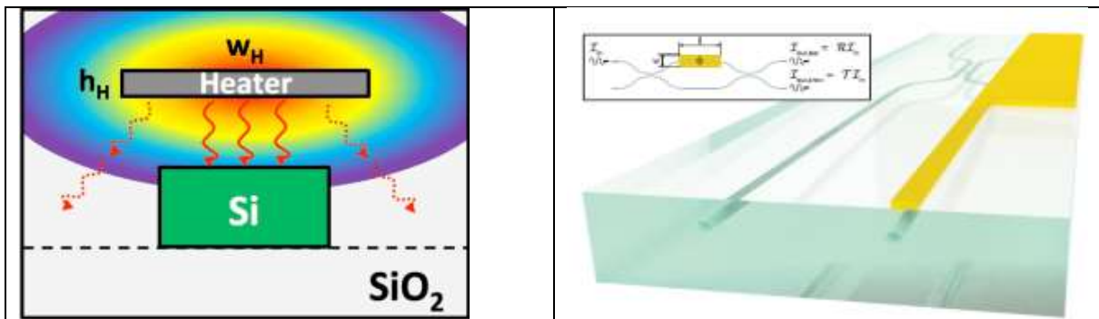
Fig. 19 (Left) Principle of the micro-heater, showing how the top electrode will diffuse heat through the Joules effect induced by the strong current passing through the metal. (Right) Example of a DLW thermo-optic beam coupler (reproduced from Ceccarelli 2019).
