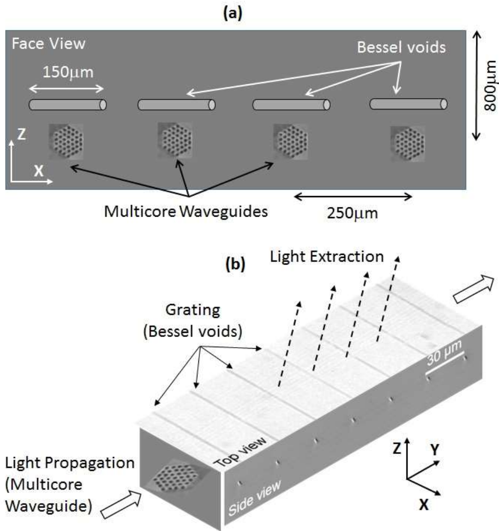
Fig. 24 (a) Face view of the whole structure showing four parallel multicore waveguides and their respective Bessel sampling centers above them. Typical dimensions are given in the figure. (b) 3D view of the device showing the disposition of the nanovoids array positioned transverse to the waveguide and the axis orientation (reproduced from d'Amico 2017)
