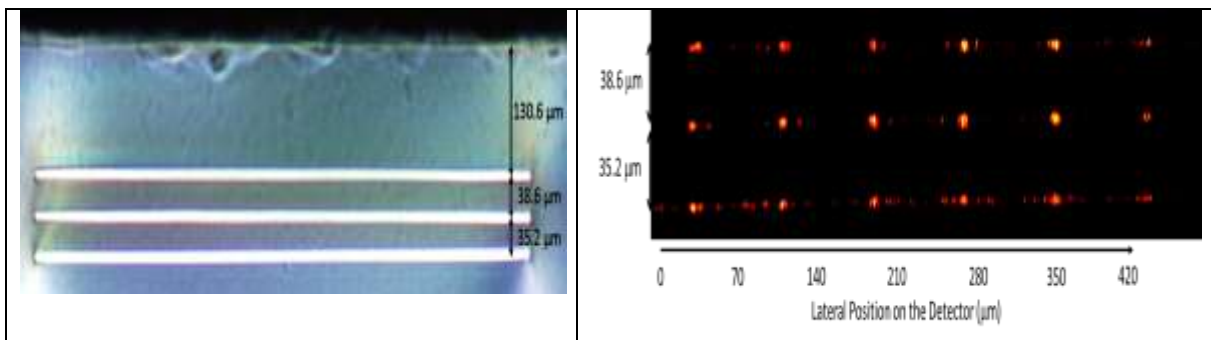
Fig. 22 ( Left ) White light image of a tri-layered AWG output facet. ( Right ) Output image of the diffracted modes, for the three layers injected simultaneously, at 790\text{nm} . (Reproduced from Douglass 2018B)
