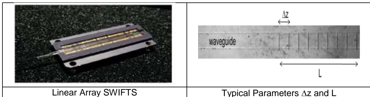
Fig. 10 Left: Image of a Visible commercial SWIFTS interferometer, showing the optical waveguide (fed by an optical fiber) glued directly to the CMOS linear detector. Right: Image of a waveguide with nano-grooves on the surface, showing the typical parameters of the sampling region (L = total sampling length and \Delta z = sampling period)
