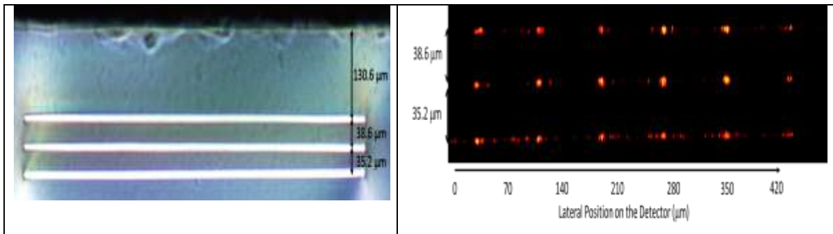
Fig. 22 ( Left ) White light image of a tri-layered AWG output facet. ( Right ) Output image of the diffracted modes, for the three layers injected simultaneously, at 790\ \text{nm} . (Reproduced from Douglass 2018B)
