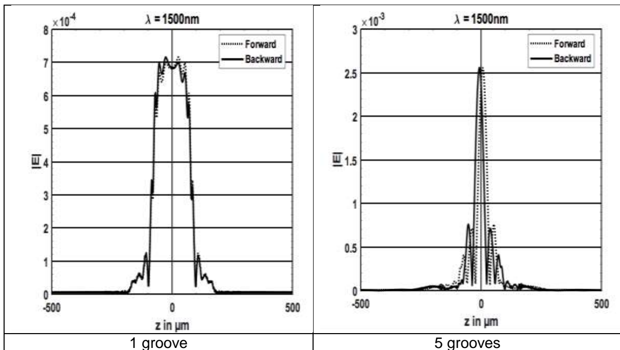
Fig. 5 Simulation of the scattered intensity profile issued from an antenna composed of N grooves at the optical wavelength 1500 nm. On the left for N=1 and on the right for N=5 (reproduced from Bonduelle 2021)
