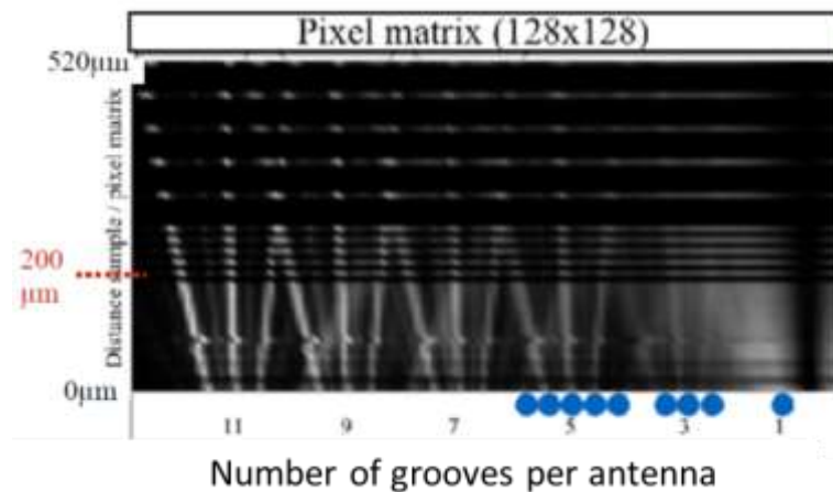
Fig. 7 Evolution of the vertical radiation pattern as a function of height between the detector and the sampling center, for different number of grooves per diffracting antenna
