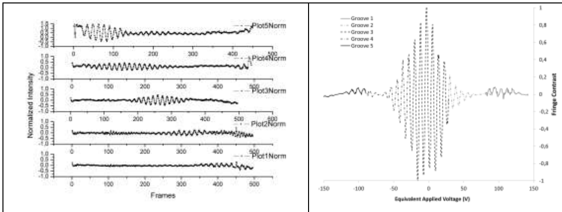
Fig 17 Example of a temporal phase shift introduced in a Lithium Niobate SWIFTS. The wide band fringes are shifted from a sampling center to the next, thanks to an applied voltage, allowing to reduce the effective sampling step, and therefore increasing the spectral range (reproduced from Loridat 2018). Note that the source must present a limited coherence length, so that an envelope can be found to identify the relative phase between scattering centers and achieve the stitching.
