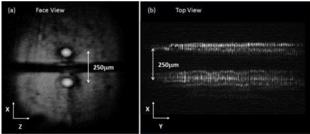
Fig. 25 Near IR observation of two parallel waveguides and the sampling centers when illuminated with a 1.56\mu\text{m} laser. (a) Direct transmission on the FLIR camera, showing the two modes of two adjacent channel waveguides. (b) Top view as signal is extracted with the sampling centers and imaged on the Goodrich Camera using a simple microscope objective (reproduced from d’Amico 2017)
