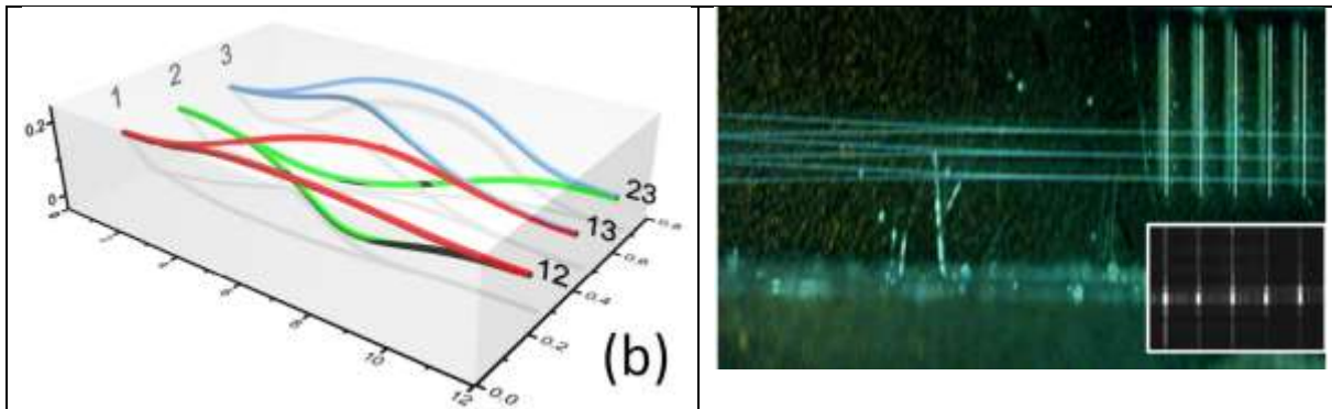
Fig. 30 (Left) Sketch of a 3D 3T beam combiner (reproduced from Rodenas 2012). (Right) Image of the fabricated 3D 3T and the sampling centers using DLW. In the inset is shown the image of the radiating sampling centers when an IR laser is injected at the input.
