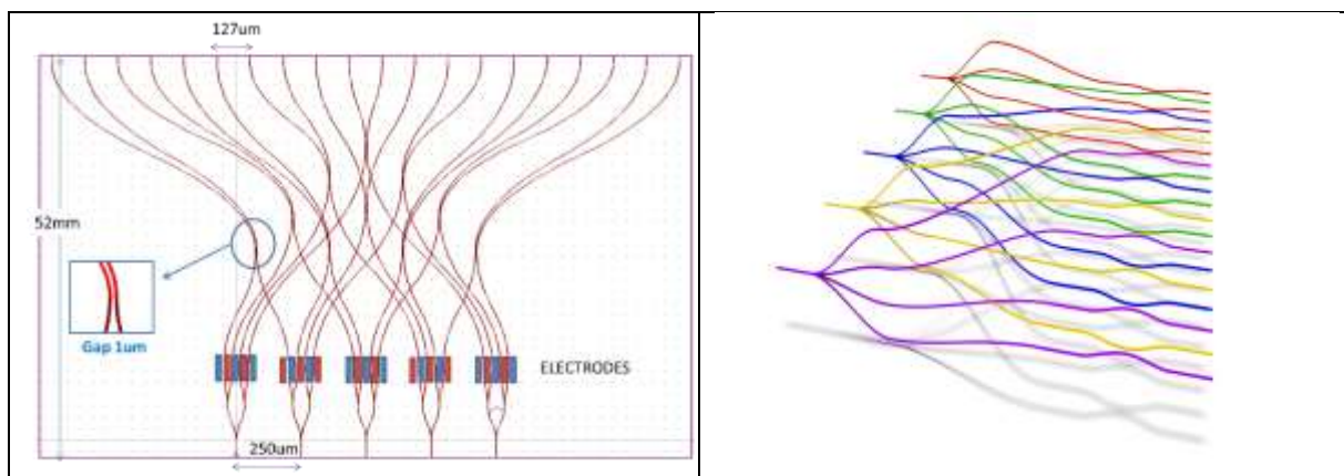
Fig. 29 (Left) Classical 2D concept of the 5T FIRST beam combiner, implying 20 parallel channel waveguides to be combined by pairs. Note the number of in-plane crossings. (Right) Concept of a
