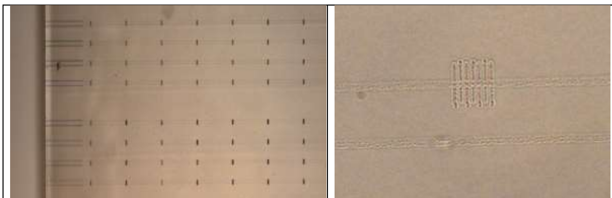
Fig. 18 (Left) Image of a set of parallel waveguides fabricated by DLW in Lithium Niobate, with the sampling centers (sets of nano-grooves) also fabricated by laser writing at the Univ.Salamanca (J. R.V. de Aldana), on the surface of the sample. (Right) Zoom on a sampling center showing the seven nano-grooves on top of the waveguide.
