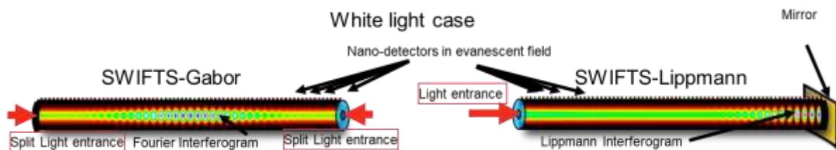
Fig. 9 Different configurations to obtain a static interferogram inside an optical waveguide: Left, counterpropagative configuration (Gabor mode); Right, Lippmann mode, using reflection at the output facet of the sample. The fringes are sampled using nano-scatterers on the evanescent field of the optical guided mode, generally on top of the waveguide.
