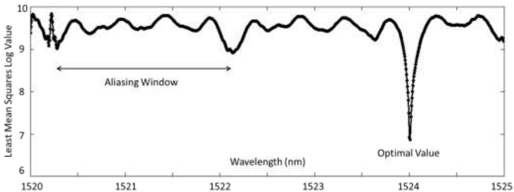
Fig. 13 Result of a least squares search for an unknown wavelength (1524.03 nm) injected on the system and comparison with the database (1524 nm), allowing for a guess wavelength with an accuracy around 25 pm.
