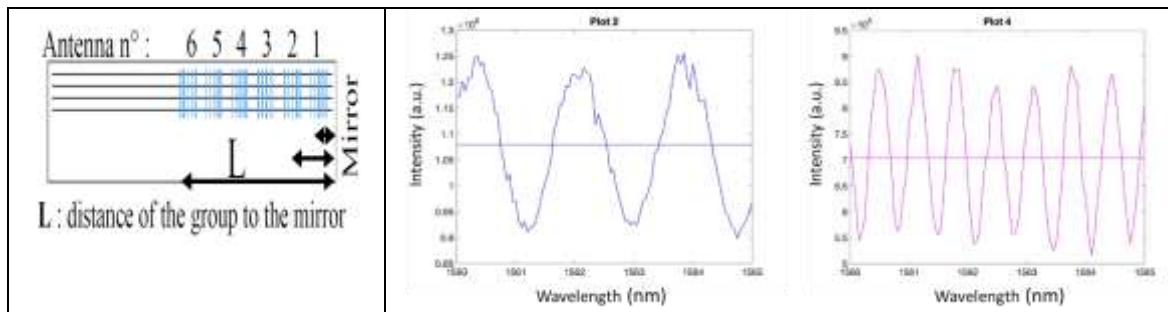
Fig. 11 Sketch of the fabricated sample, showing different sets of nano-scattering centers (Bessel voids) at different distances from the mirror. All scattering centers consist of 5 Bessel voids, to improve flux directivity. On the right, the sampled intensity for antennas number 2 and 4 respectively, showing the influence of the distance to the mirror on the frequency of the fringes (reproduced from Bonduelle 2020).
