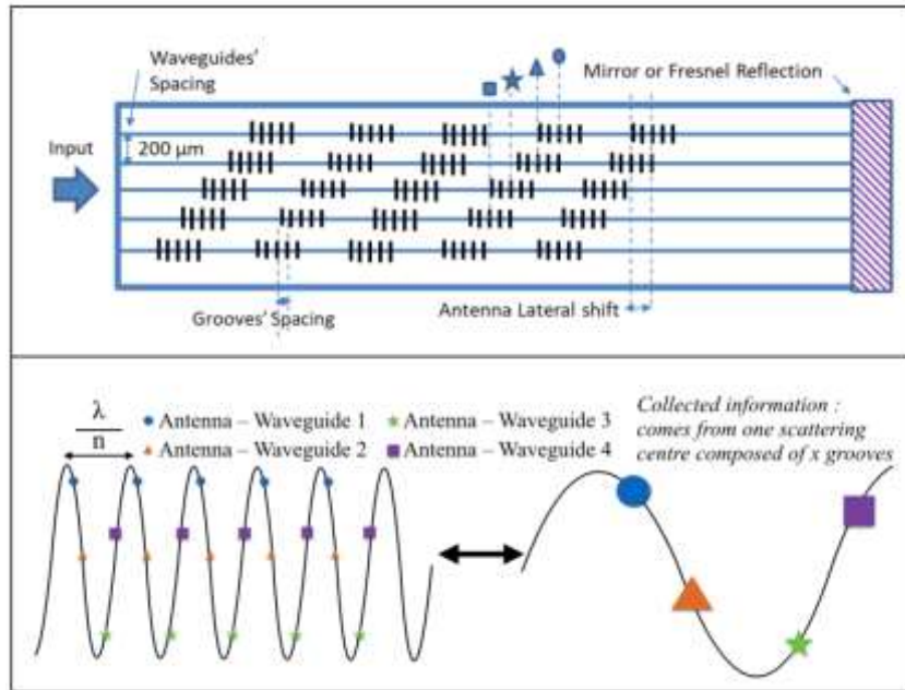
Fig. 14 Sampling with a spatial offset. Each antenna is set at a different length from the reflecting mirror, sampling a different part of the interferogram. After stitching, an improved sampling of the interferogram is obtained (reproduced from Bonduelle 2021).
