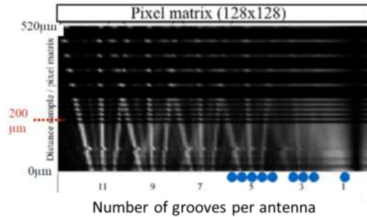
Fig. 7 Evolution of the vertical radiation pattern as a function of height between the detector and the sampling center, for different number of grooves per diffracting antenna
