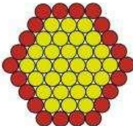
Core-Shell
