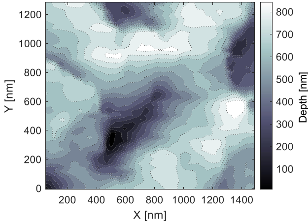
Figure 4: Surface topography of “worm-like” nanostructures as observed by atomic force microscopy.
