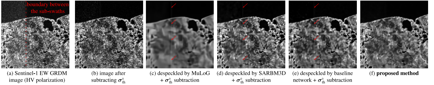
Figure 8. Application to an actual Sentinel-1 EW GRDM image (HV polarization channel) of an area in Northern Russia (©ESA): (a) original image; (b) after correcting for the thermal noise bias; (c-e) restored image by despeckling image (a) and subtracting the thermal a posteriori ; (f) proposed method: restoration of image (b) with a network aware of the thermal noise map \sigma_{th}^0 . Artifacts pointed by red arrows are visible at the boundary between the sub-swaths indicated by the vertical dashed line in (a) for methods (c-e) and are almost absent of the result (f).
