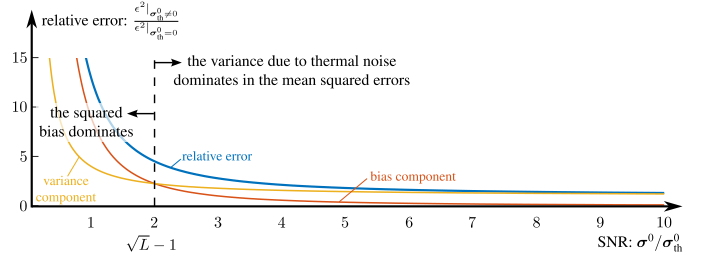
Figure 4. Impact of the thermal noise on the radar intensities: evolution of the relative mean squared errors \epsilon^2 with the signal-to-noise ratio, as established in equations (10) and (11).
