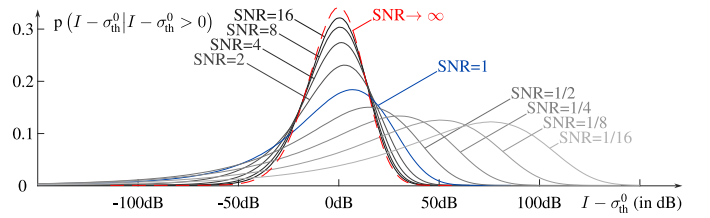
Figure 6. After compensation of the shift due to the thermal noise floor, corrected intensities follow a different statistical distribution. Here, the probability density function of the corrected intensities is represented, in log scale (dB), for different SNR values (ratios of the reflectivity and the thermal noise floor \sigma_{th}^0 ). Compared to the Fisher-Tippett distribution followed in the absence of thermal noise correction (red dashed curve, \text{SNR} \rightarrow \infty ), the shape of the distribution is strongly modified by the correction, preventing from directly applying despeckling methods to corrected images.
