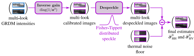
Proposed: correct thermal bias, then despeckle while accounting for the modified speckle distribution.
